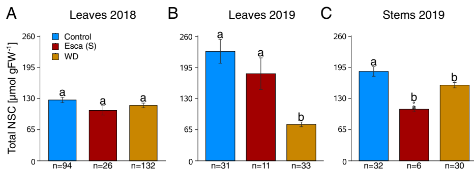
Fig. 4. Total NSC content in \mu\text{mol} \cdot \text{gFW}^{-1} over the 2 y for control (blue), esca-symptomatic (red), and WD ( \Psi_{\text{PD}} < -0.5 MPa, yellow) leaves and stems. (A) Mean NSC content in leaves in 2018. (B) Mean NSC content in leaves in 2019. (C) Mean NSC content in stems in 2019. Bars represent means and error bars SEs; letters indicate statistical significance ( P < 0.05 ) from independent mixed linear general models with Tukey's post hoc comparisons (SI Appendix, Tables S2 and S3). Sample sizes (n) are presented below each bar, and individual data points (dots) are presented for bars with sample sizes \leq 10 .
